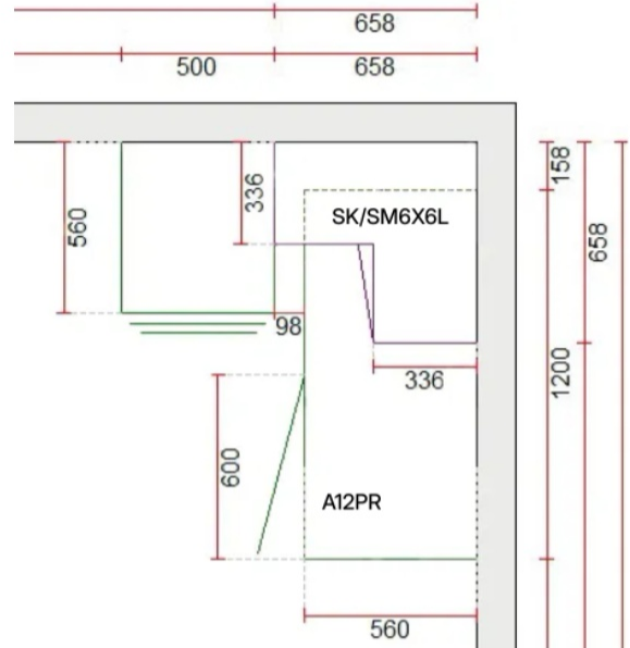
6. Blind corner dimensioning: 1200 mm with 596 mm door
