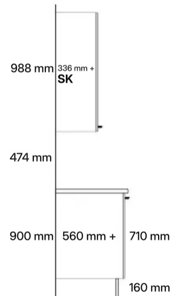
Side profile 2362 mm
