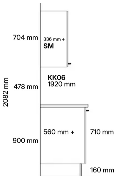
Side profile 2082 mm
