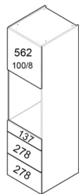
OVEN WITH 3 DRAWERS
