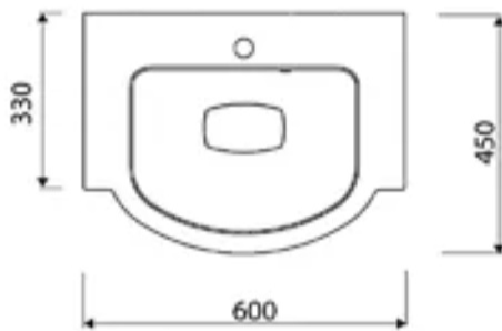
LEFT-HANDED BASIN
